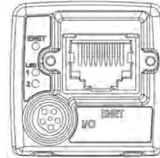
In-Sight 8405
